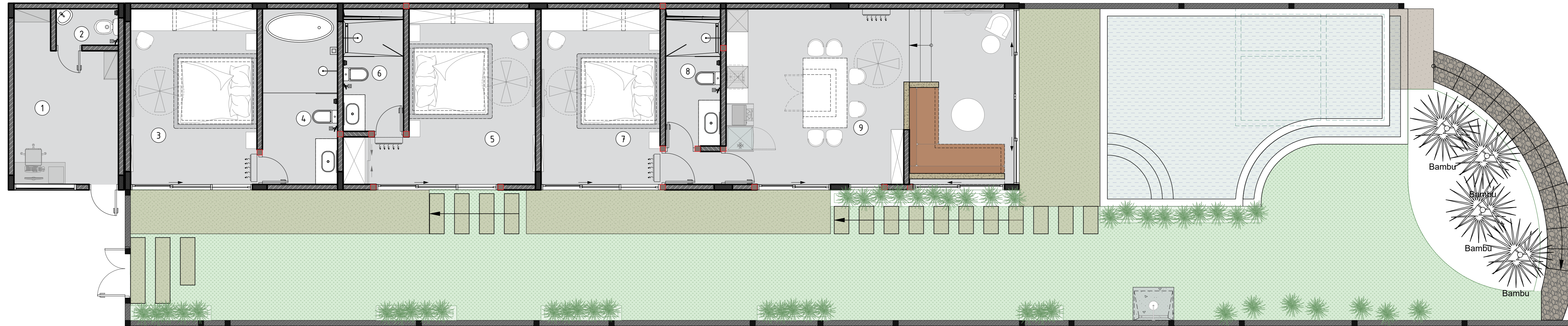
Ground floor plan. LOT 3.
