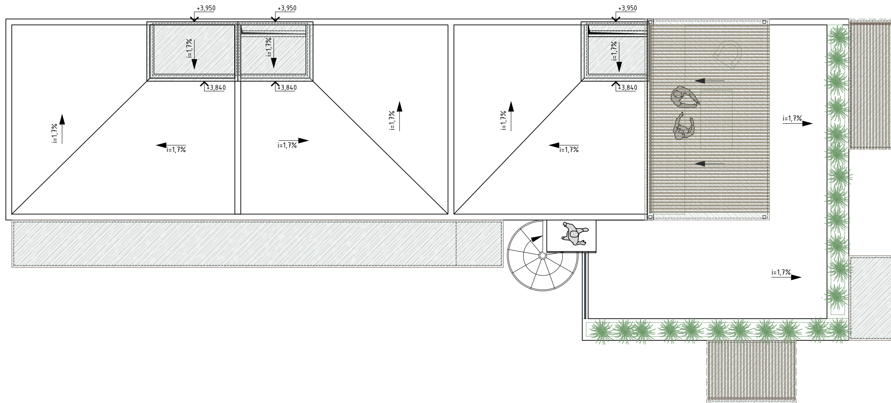
Rooftop plan. LOT 1.
